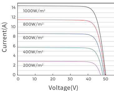
Current-Voltage Curve JAM72D30-575/LB/1500V
